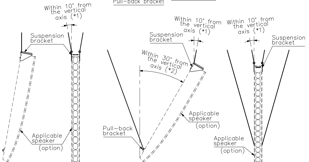
Two-wire suspension method
